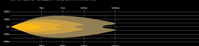
LR-24 ELITE+ (YELLOW ONLY) SNOW / FOG / DUST MODE
