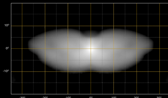
LR-24 ELITE+ (WHITE ONLY) E-BOOST MODE
