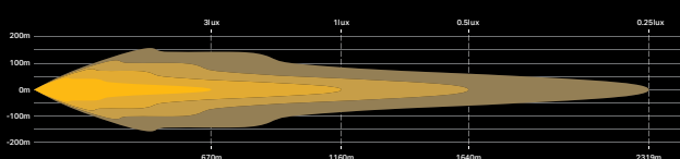
LR-24 ELITE+ (WHITE AND YELLOW) COMBO MODE
